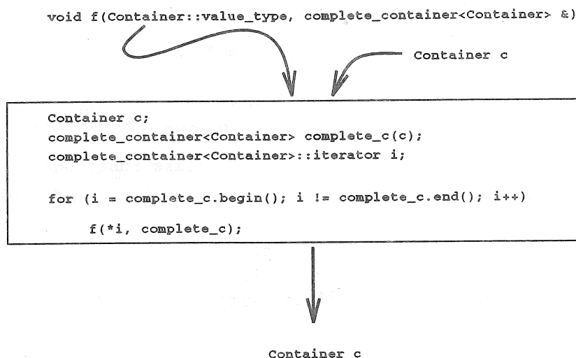
Figure 2: Implementing complete traversals by using a container adaptor approach
